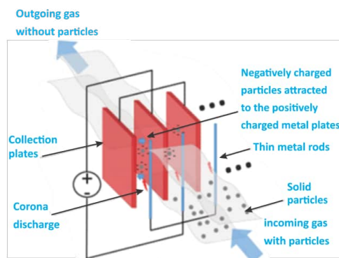
Fig. 15.11: Electrostatic precipitator
