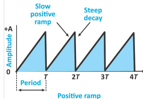
Fig. 18.12: Schematic diagram of a saw-tooth wave
