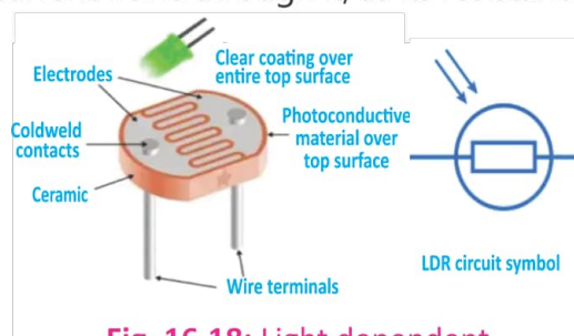
Fig. 16.18: Light dependent resistor
