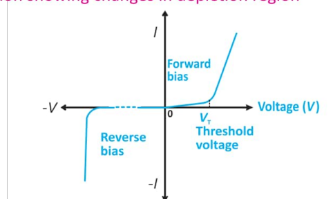
Fig. 19.5: I - V graph of a semiconductor diode
