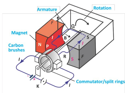
Fig. 17.9: Working principle of D.C motor
