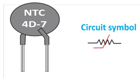
Fig. 16.17: NTC thermistor
