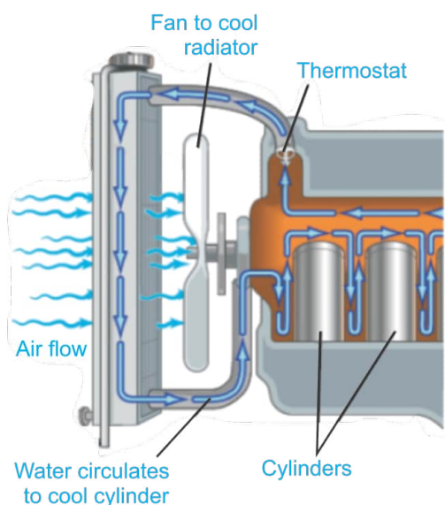
Fig. 10.7: Cooling system of automobile
