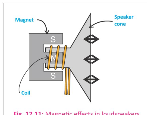
Fig. 17.11: Magnetic effects in loudspeakers
