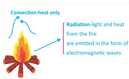
Fig. 11.10: Thermal radiations transform in form of E.M waves
