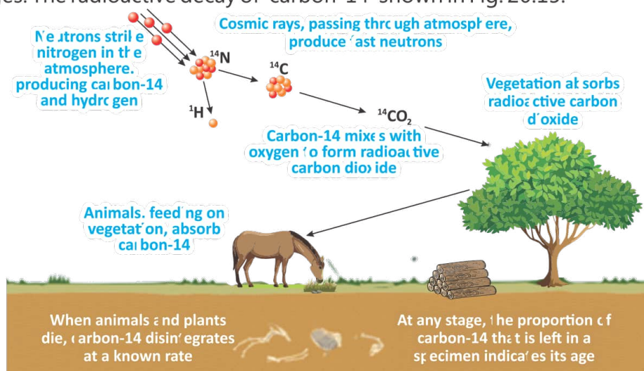
Fig. 20.15: Carbon dating
