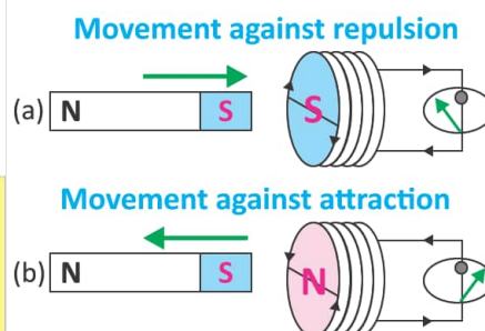
Fig. 18.4: Lenz's law
