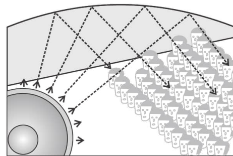
Fig. 13.16(b): Curved ceiling of a conference hall
