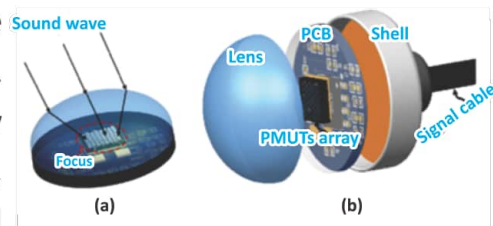
Fig. 14.28: Diagram of acoustic lens
