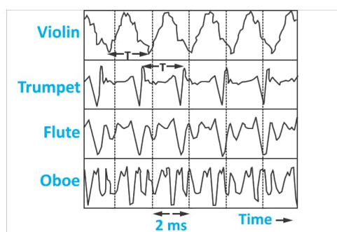
Fig. 13.9: Oscilloscope traces of different sound sources
