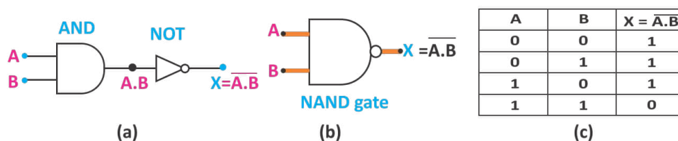
Fig. 19.17 (a,b): The circuit symbol (c) Truth table for NAND gate
