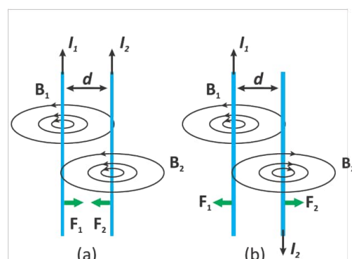
Fig. 17.5: Forces between parallel wires
