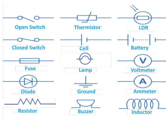
Fig. 16.23: Symbols of various electrical components
