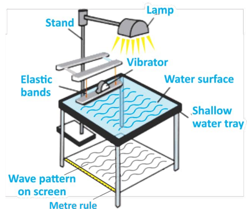
Fig. 12.5: Ripple tank
