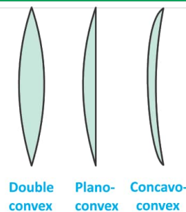
Fig. 14.12: Convex lenses
