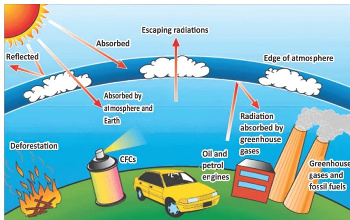
Fig. 21.5: Illustration of global warming
