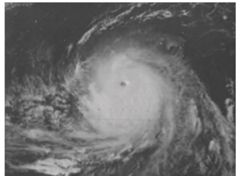
Fig. 21.6: Hurricane
