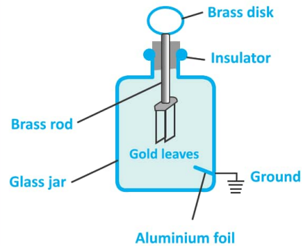
Fig. 15.7: Uncharged electroscope
