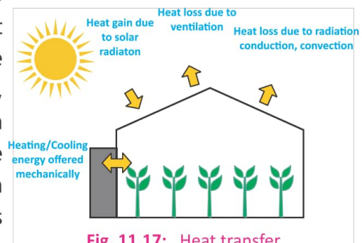
Fig. 11.17: Heat transfer mechanisms in a greenhouse
