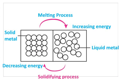
Fig. 10.8: Phase changes
