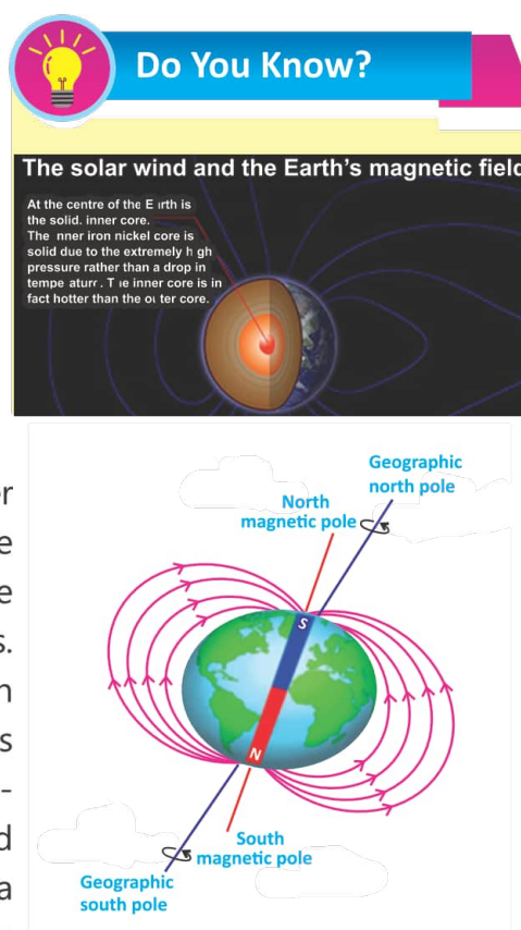
Fig. 17.13: Origin of Earth's magnetic field
