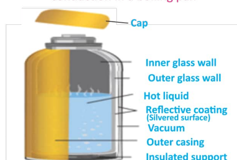
Fig. 11.15: Thermos flask
