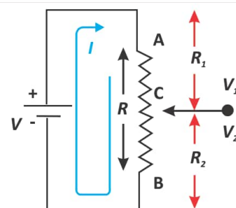
Fig.16.15: Potential divider circuit
