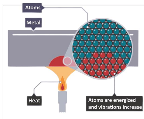
Fig. 11.1: Heat transfer in metals through conduction
