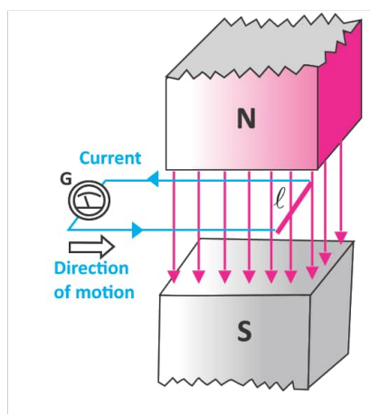
Fig. 18.2: Induction of current by moving a wire through a magnetic field
