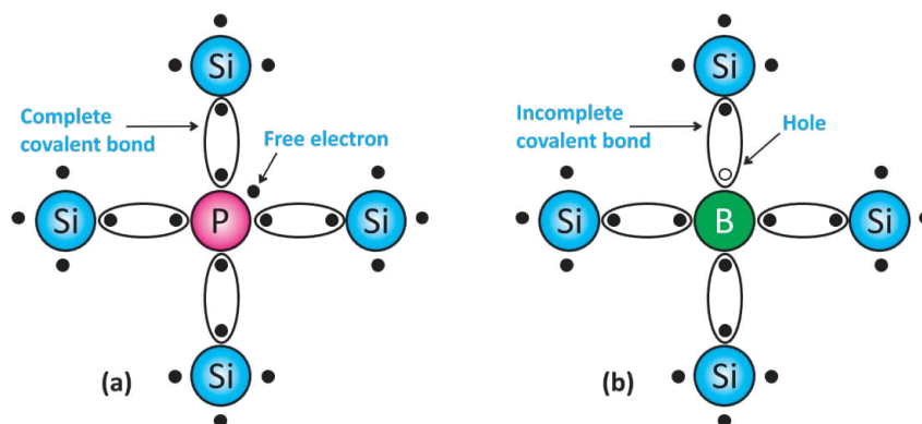
Fig. 19.1: (a) N-type semiconductors (b) P-type semiconductors
