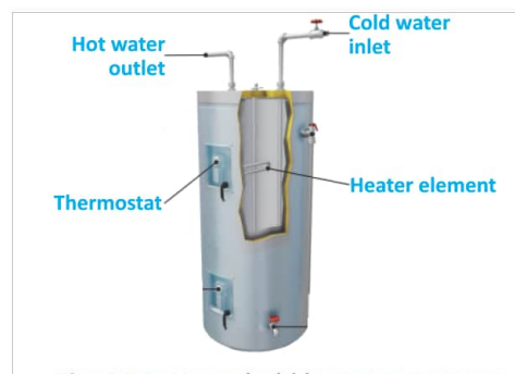
Fig. 11.9: Household hot-water system
