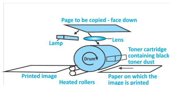
Fig. 15.10: Labelled diagram of a multifunction photocopier machine
