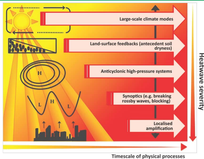
Fig. 21.7: Heatwave schematic illustrating the various physical processes
