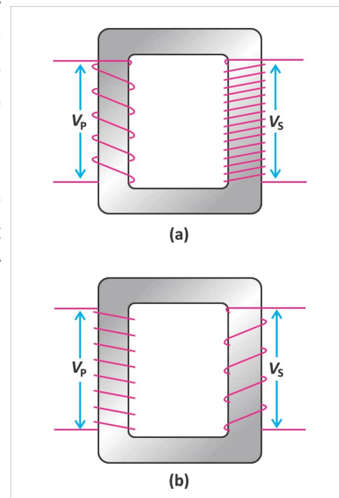
Fig. 18.8: (a) Step-up transformer (b) Step-down transformer
