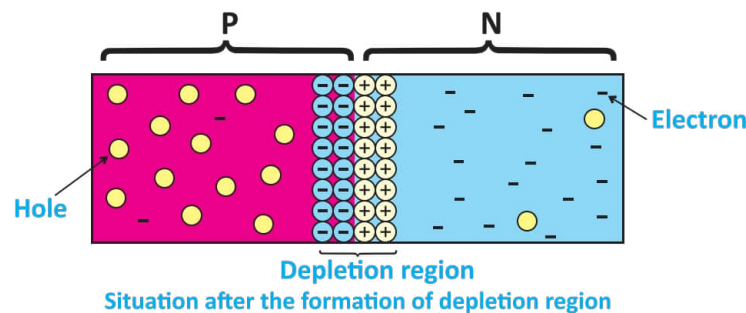
Fig.19.2: Schematic diagram of formation of PN junction
