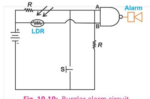
Fig. 19.19: Burglar alarm circuit using NAND gate
