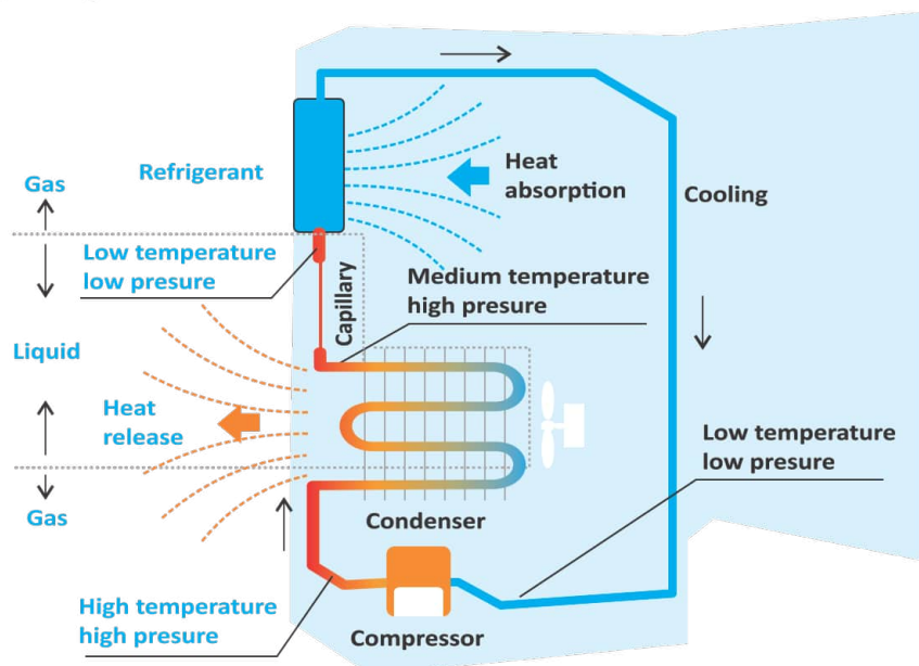
Fig. 10.11: Block diagram of refrigerator
