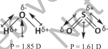
Figure 3.6 Vector addition of individual bond moments in angular \text{H}_2\text{O} and \text{SO}_2 molecules
