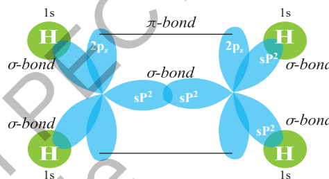
Figure 11.8 Bond formation of carbons in ethene
