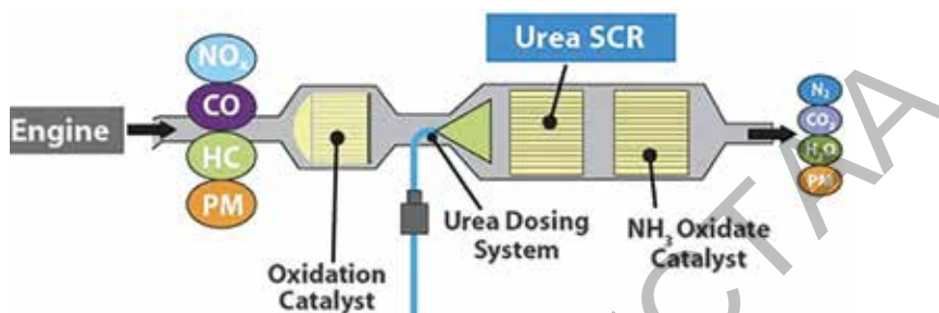
Figure 14.6 Selective Catalytic Reduction
