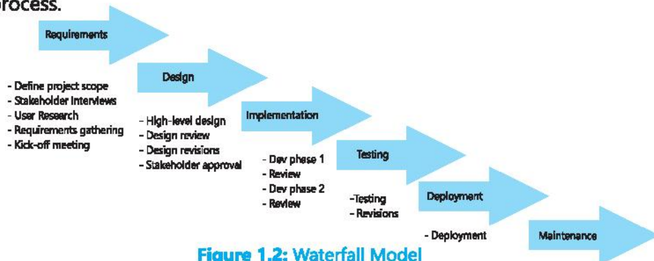
Figure 1.2: Waterfall Model
